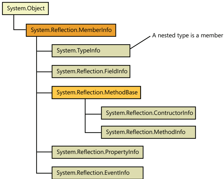
FIGURE 23-1 Hierarchy of the reflection types that encapsulate information about a type's member.
