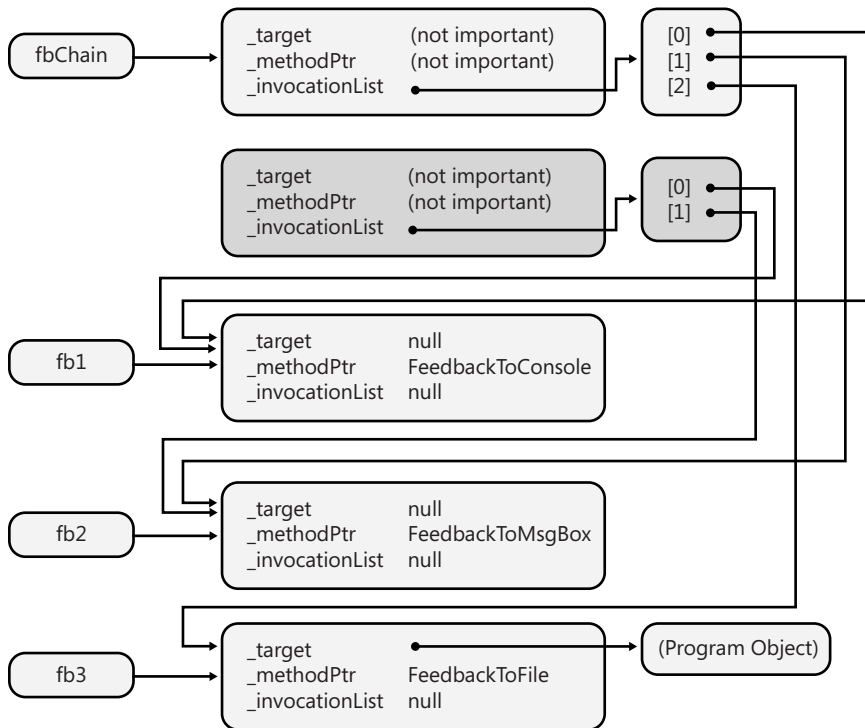
FIGURE 17-6 Final state of the delegate objects when the chain is complete.
