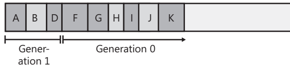
FIGURE 21-6 New objects are allocated in generation 0; generation 1 has some garbage.
