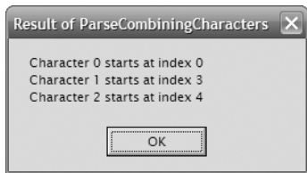
FIGURE 14-4 Result of ParseCombiningCharacters .
