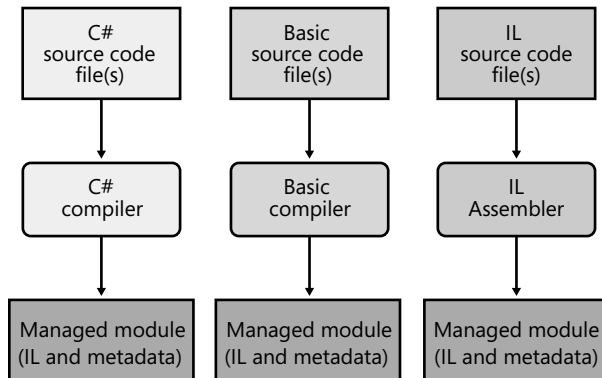
FIGURE 1-1 Compiling source code into managed modules.
