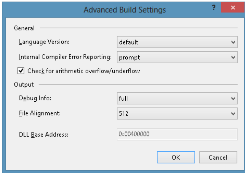
FIGURE 5-1 Changing the compiler's default setting for performing checked arithmetic using Visual Studio's Advanced Build Settings dialog box
