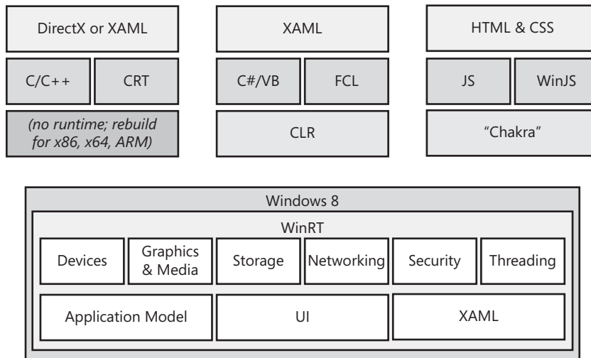
FIGURE 25-1 The kinds of features exposed by Windows' WinRT components and the various languages that Microsoft supports to access them.
