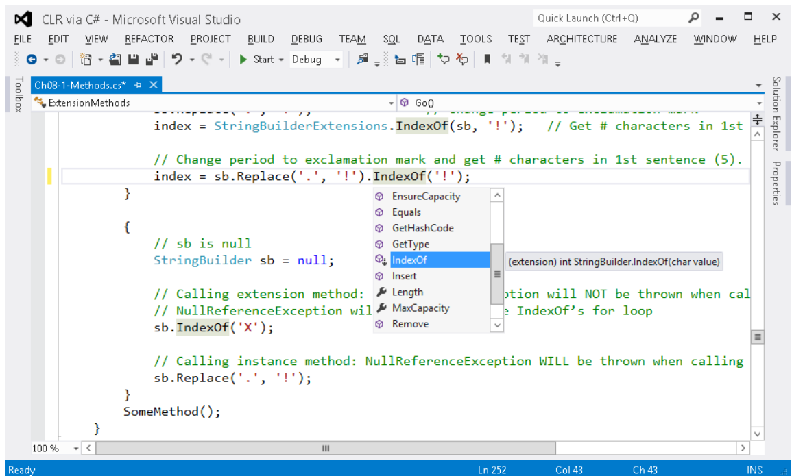
FIGURE 8-1 Visual Studio's IntelliSense window, showing extension methods.
